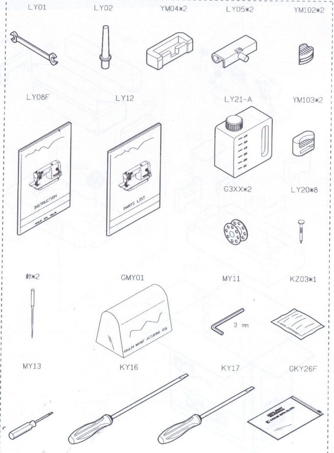
PARTS LIST FOR LY GROUP
