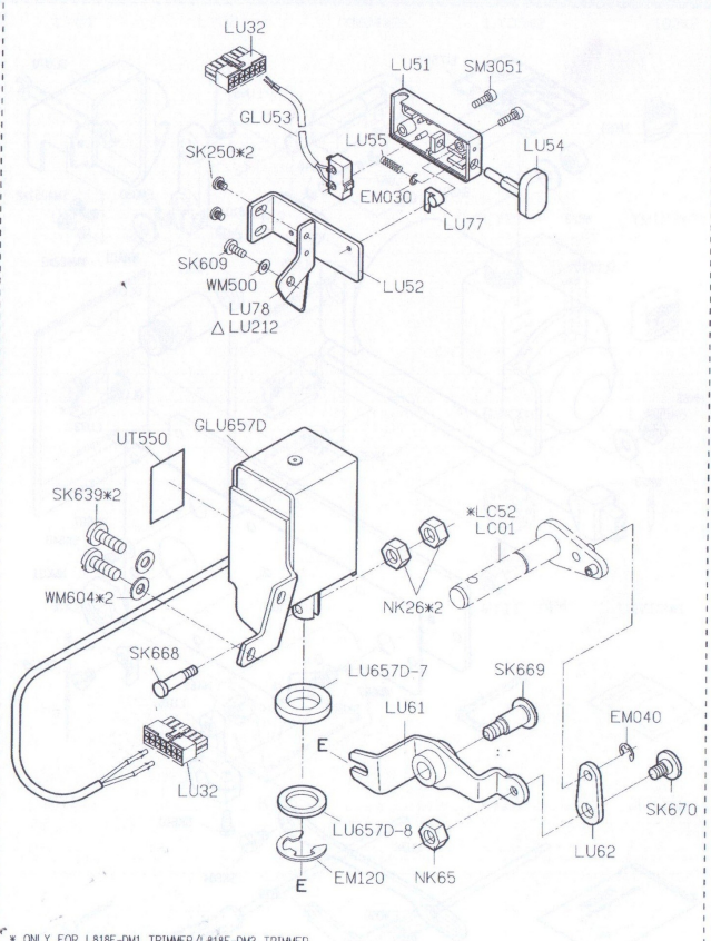
PARTS LIST FOR LU (3) GROUP
