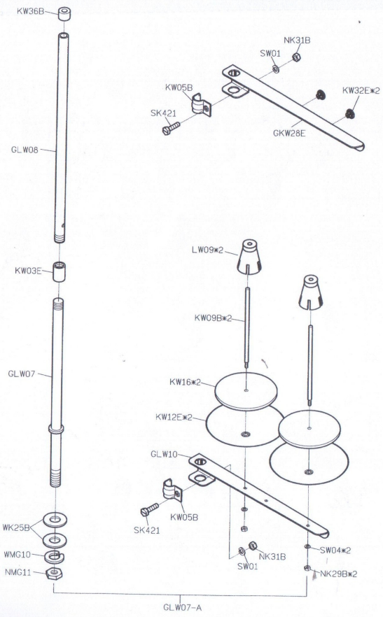
PARTS LIST FOR THREAD STAND GROUP
