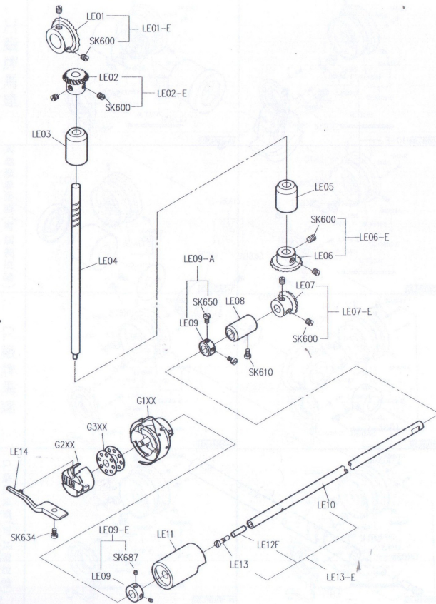
PARTS LIST FOR LE GROUP
