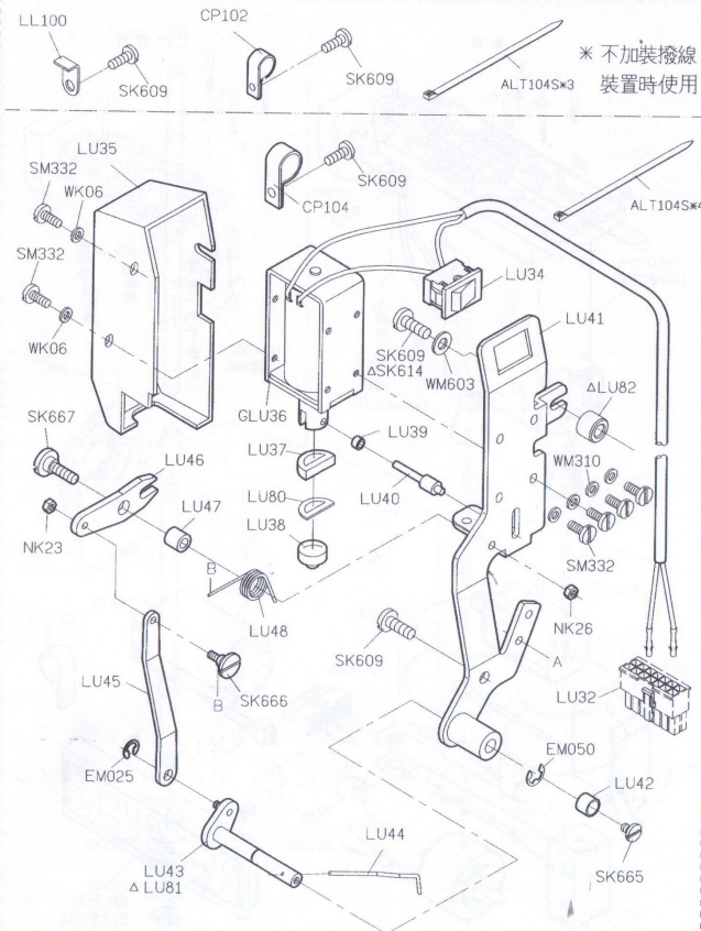
PARTS LIST FOR LU (2) GROUP
