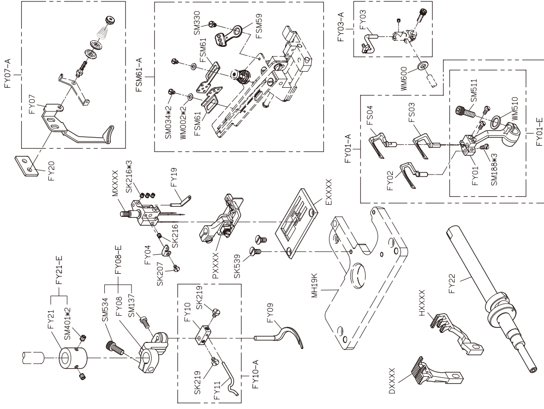
FOR F007K/F007KD/F858K/F858KD
