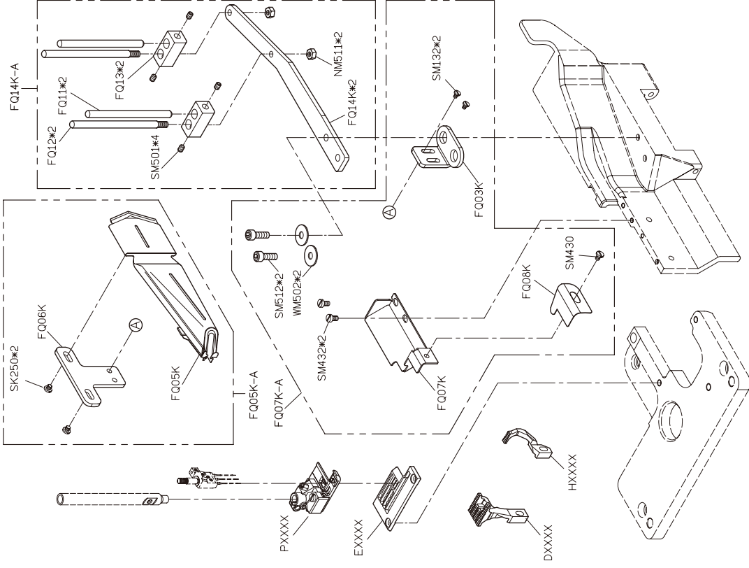
FOR F007K/F007KD/F858K/F858KD
